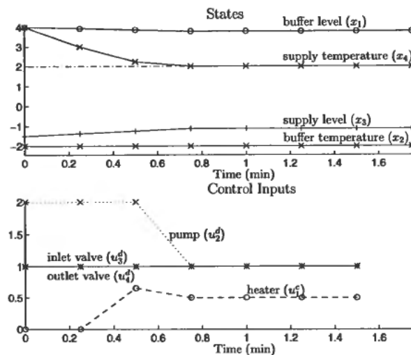
Figure 7. Integrated Design . For an explanation of the vertical axes, see Fig. 4.
