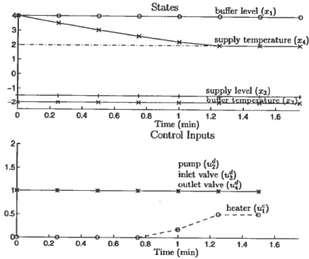
Figure 4. Separate Design I . The vertical axis in the upper part of the figure has the following interpretation: The zero point corresponds to 20°C and 3 meters for the temperature and levels respectively, and the scaling is 1°C and 1 meter respectively. The dash-dotted line is the setpoint ( x_{40} ) for the supply temperature. Further, the vertical axis in the lower part of the figure has the following interpretation: The zero point corresponds to no heating, pump stopped, and closed valves. 1 corresponds to full heating ( 2u_{10} ), pump running on stage 1, and open valves. 2 corresponds to pump running on stage 2.
