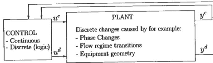
Figure 1. Process control. u^c denotes the continuous control inputs, u^d denotes the discrete control inputs, y^c denotes the continuous outputs, and y^d denotes the discrete outputs.
