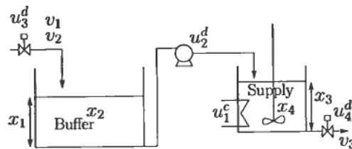
Figure 2. Two-tank system.
