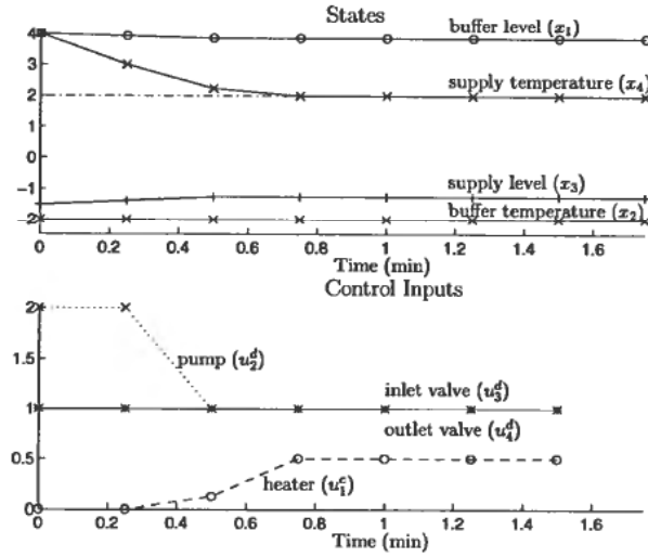
Figure 6. Full MPC. For an explanation of the vertical axes, see Fig. 4.
