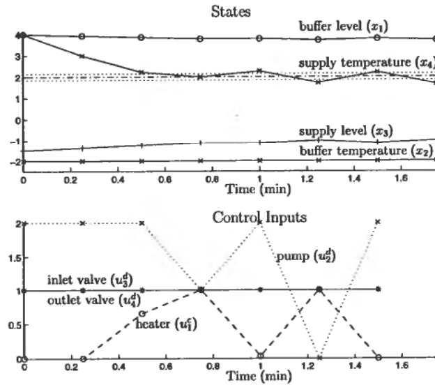
Figure 5. Separate Design II . For an explanation of the vertical axes, see Fig. 4.
