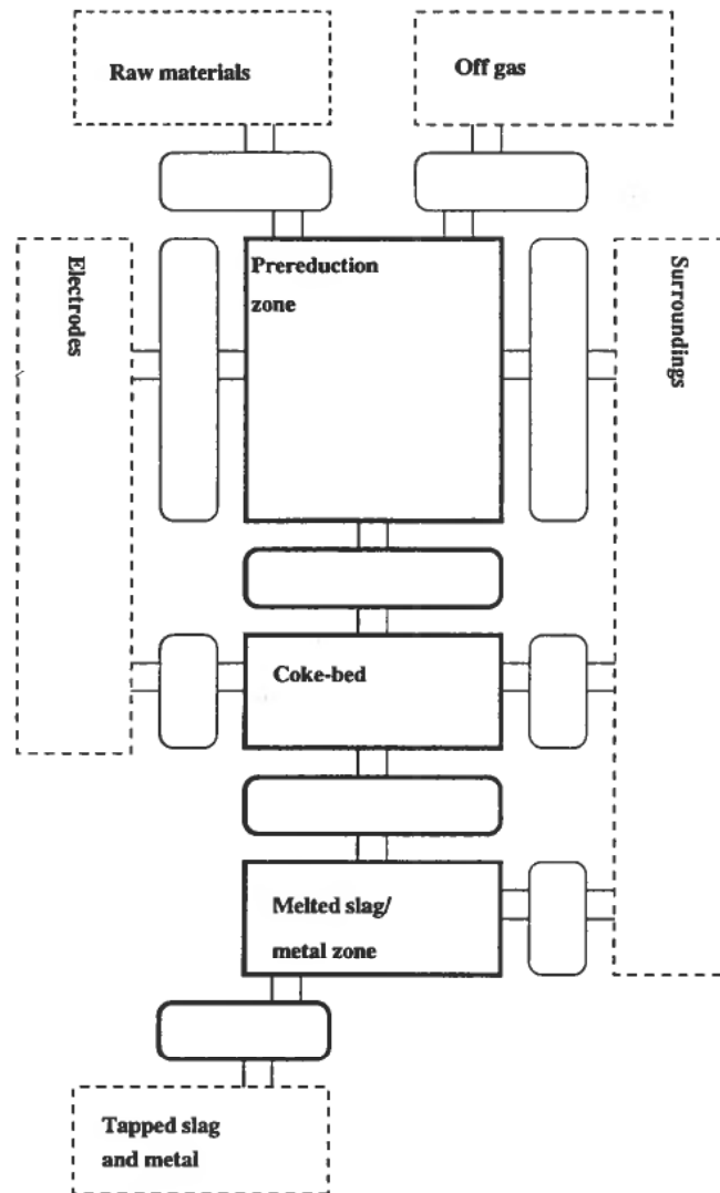
Figure 6. Sketch of the shaft model.
