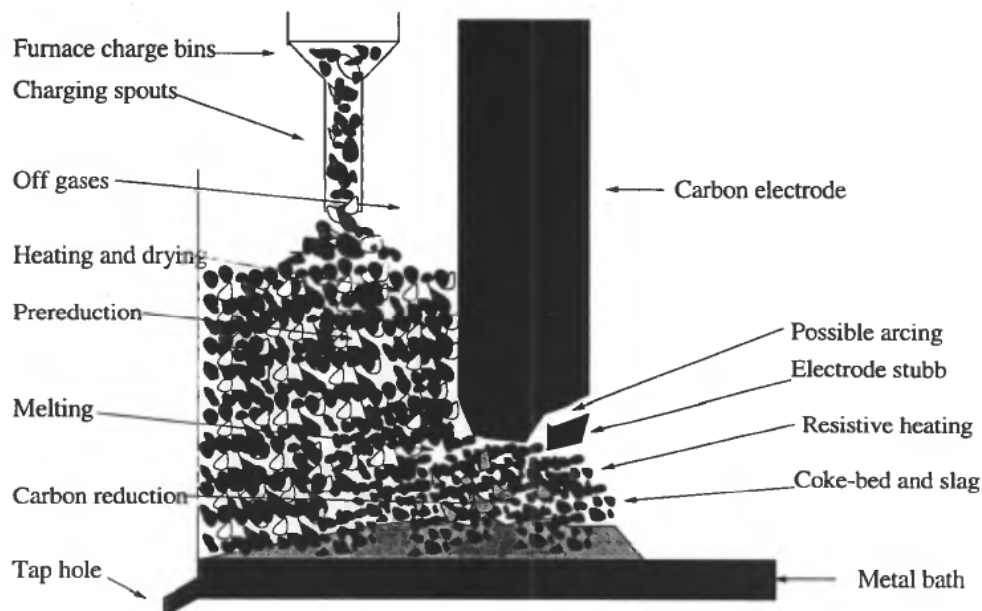
Figure 5. Sketch of the metallurgical system of a HC-FeMn furnace.
