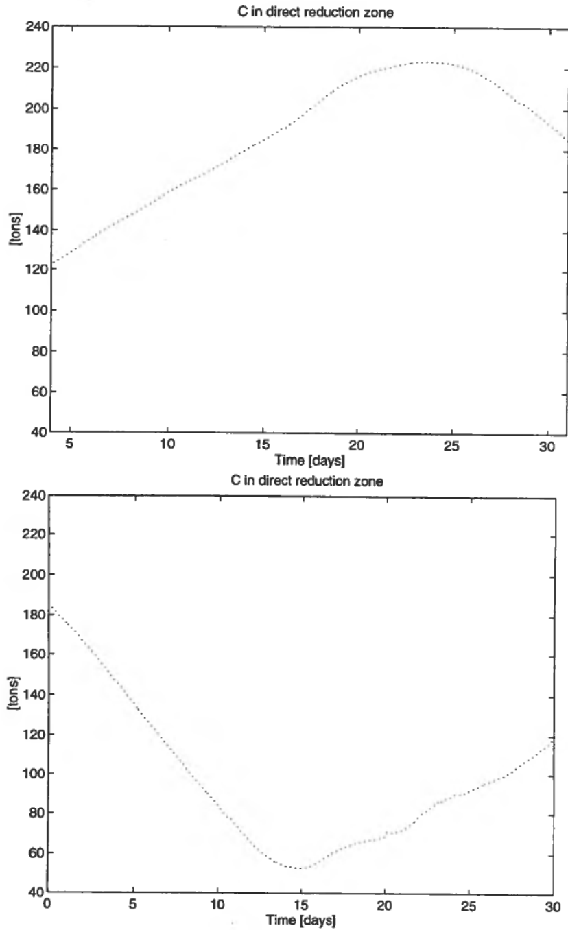
Figure 9. Accumulated carbon in the coke-bed. October 1993 (left) and November 1993 (right).
