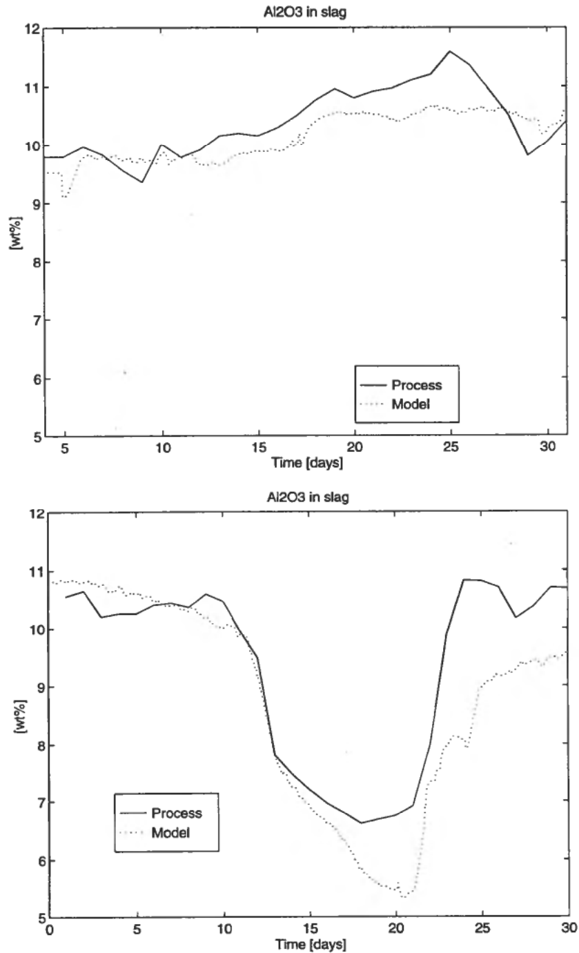
Figure 8. Model validation: Al_2O_3 in the slag. October 1993 (left) and November 1993 (right).
