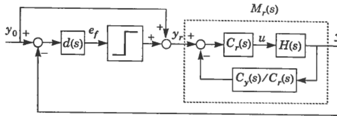
Figure 1. Block diagram showing the relay feedback path from the process measurement, y , to the reference signal for the controller, y_r .
