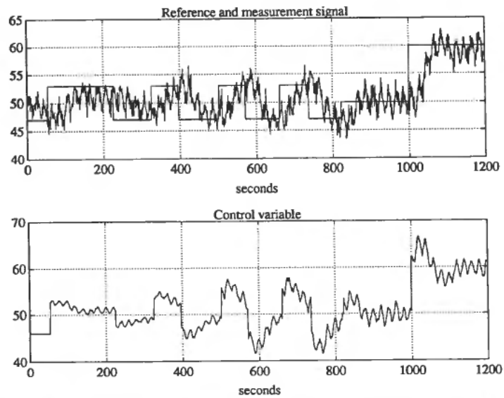
Figure 5. Autotuning of PI controller for process with measurement noise and periodic disturbance.
