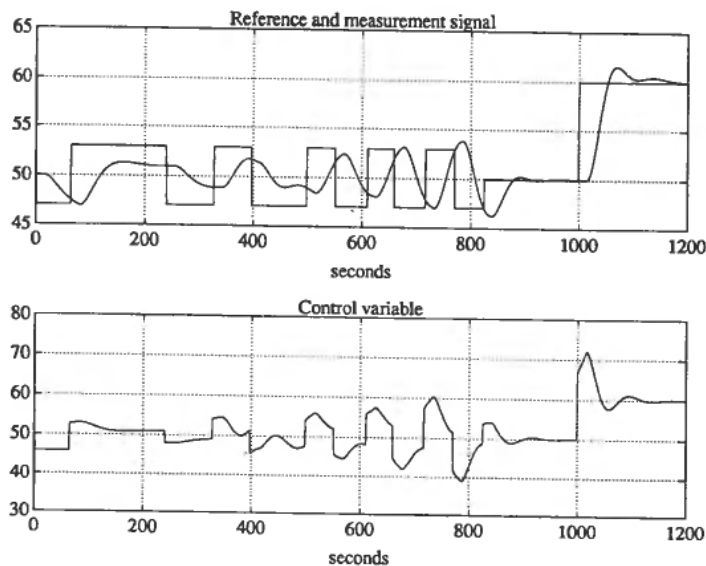
Figure 3. Autotuning of PID controller. The tuning is terminated after about 850 seconds. After 1000 seconds there is a step in the reference signal for the controller.
