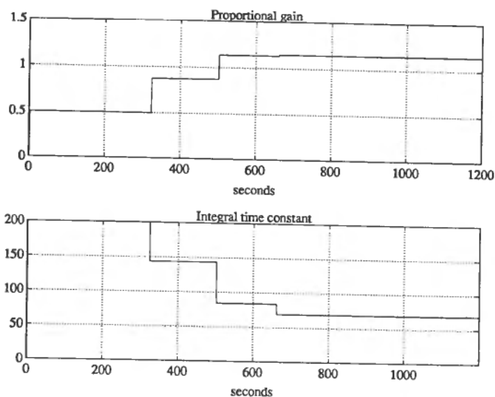
Figure 6. Proportional gain and integral time constant during tuning of PI controller in Fig. 5.
