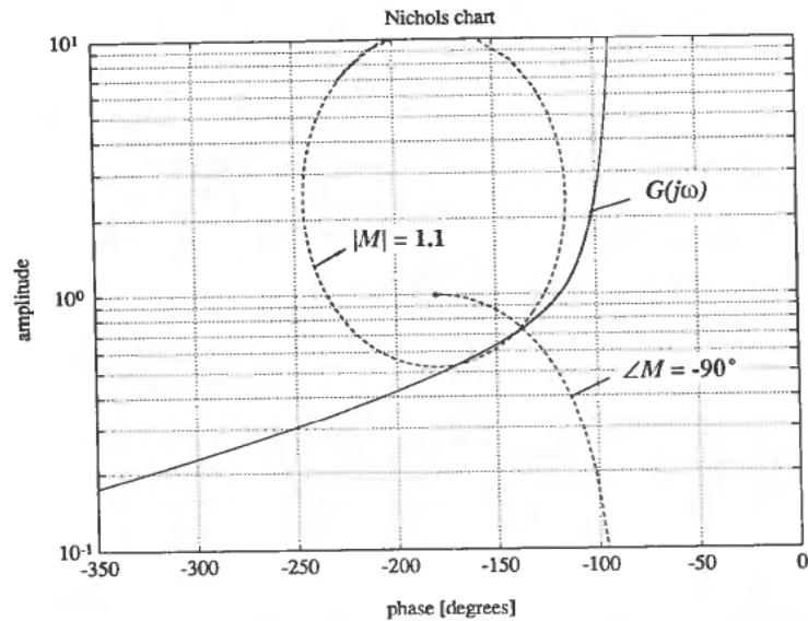
Figure 2. Nichols chart for determination of the complementary sensitivity function. Only the curves for |M|=1.1 and \angle M=-90^\circ are shown on the chart. The frequency and the amplitude of the limit cycle oscillation are determined by the intersection of the loop transfer function G(j\omega) and the curve for \angle M=-90^\circ .
