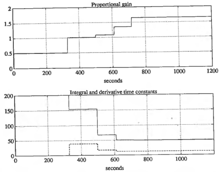
Figure 4. Proportional gain, integral time constant and derivative time constant (dashed line) during tuning of PID controller in Fig. 3. Initially the controller has only proportional action ( T_i = \infty and T_d = 0 ).
